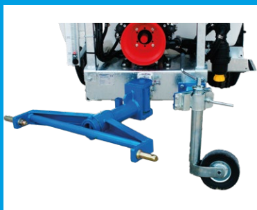
STEERING SHAFT
